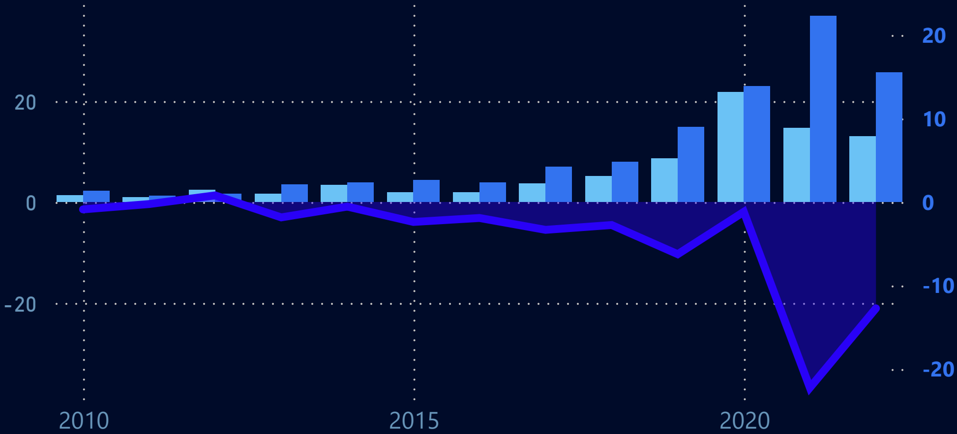
Apple Microsoft Volatility Difference
